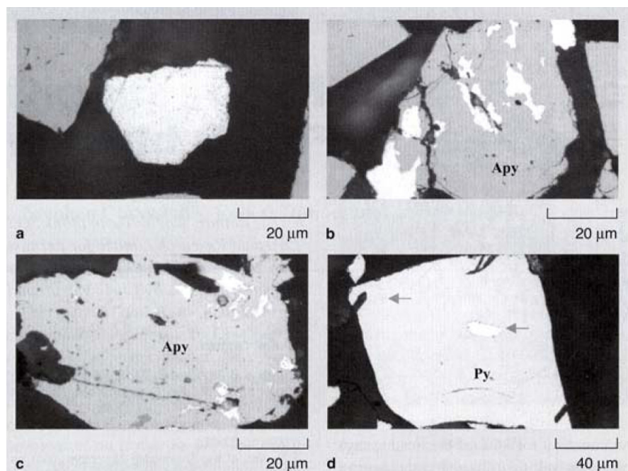
Figure 2. Photomicrographs showing the mode of occurrence of microscopic gold. (a), liberated; (b) and (c), attached to and locked in arsenophy (Apy); and (d), locked in pyrite (Py).
