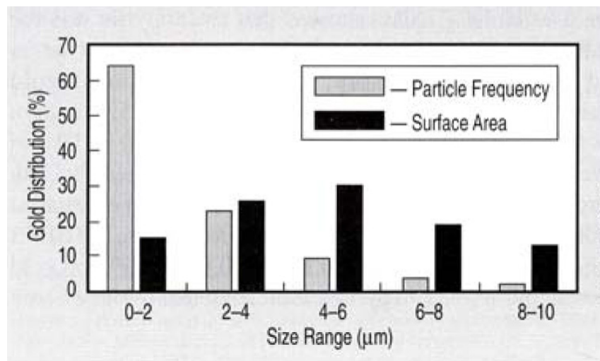
Figure 4. The size distribution of gold locked in sulfide minerals. Finer grinding is required to recover these inclusions.
