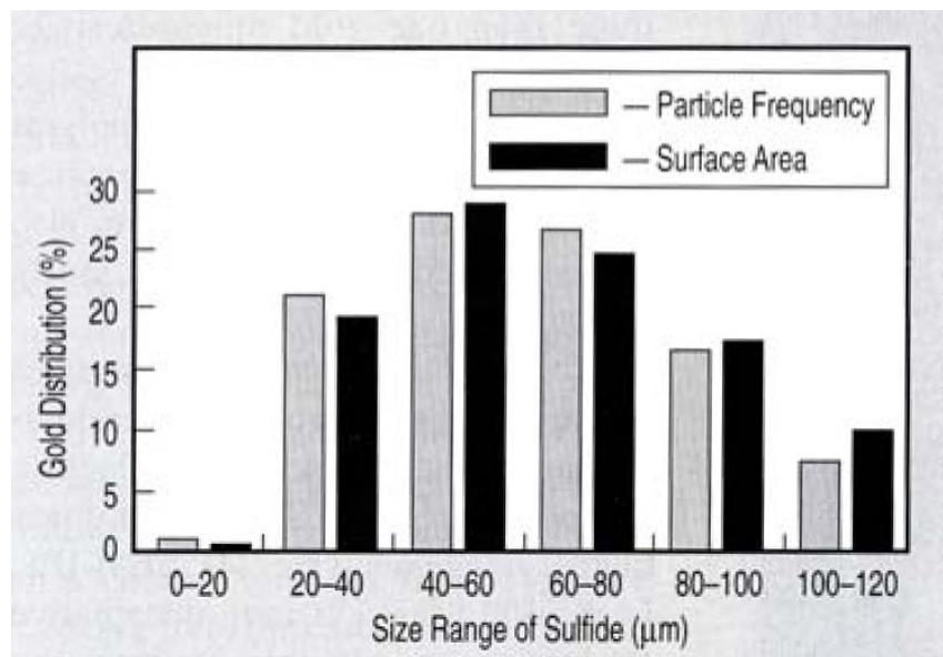
Figure 5. The distribution of locked gold vs. size of gold-bearing sulfide minerals. The majority of gold-bearing sulfide minerals ranged from 20 \mu\text{m} to 100 \mu\text{m} (accounting for ~90% of total particles and surface area), indicating that 20 \mu\text{m} of regrinding fineness will be required to liberate or expose the gold inclusions locked in sulfide minerals.
