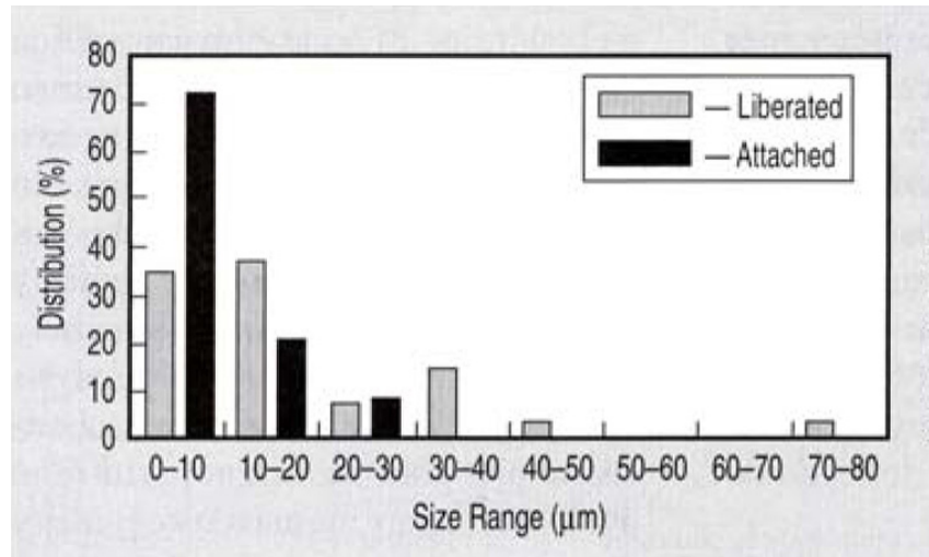
Figure 3. the size distribution of liberated and attached gold particles. the majority of gold particles were less that 40 \mu\text{m} in size.
